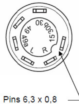
Connectors
