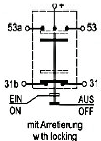
Circuit diagram
