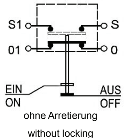
Circuit diagram
